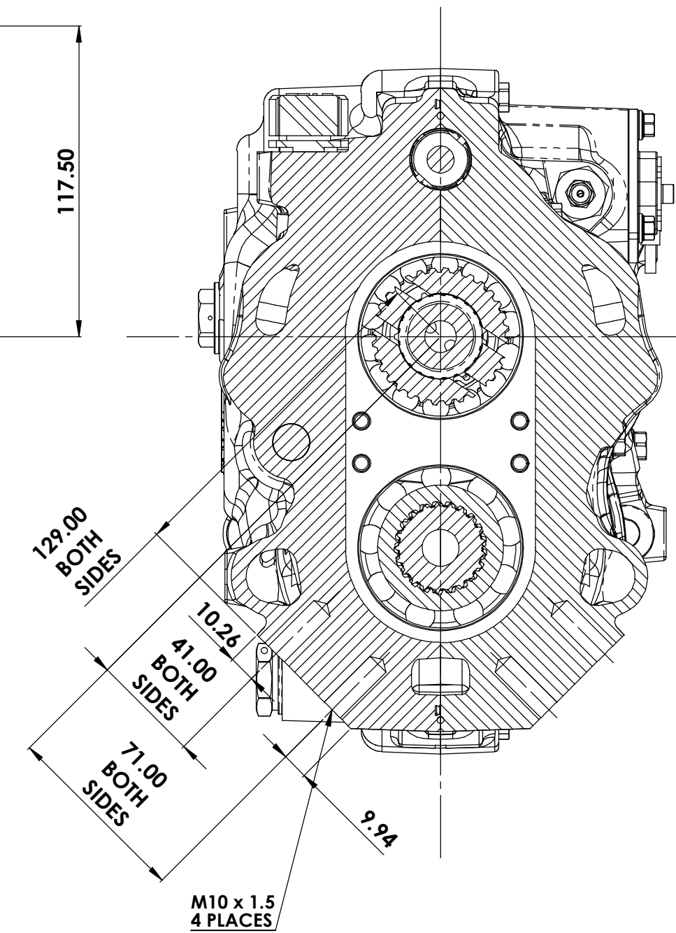
SECTION B-B
